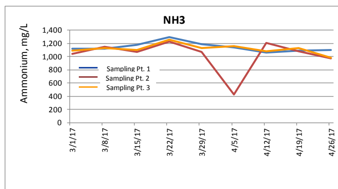
Figure 5. Ammonium Concentration Profile
